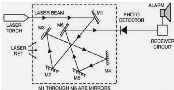
Fig. 3. Use of mirrors to form a mesh of laser beam
