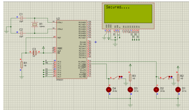
Fig.11. No Intruder Detected
