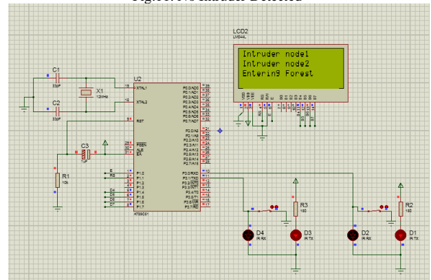
Fig.12. Intruder Entering Forest is detected
