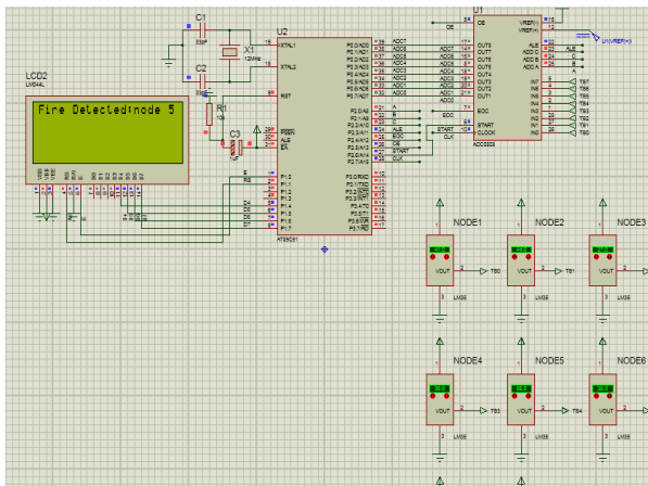
Fig. 8. Fire detected at node 5
