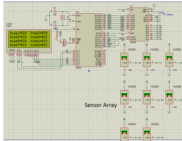
Fig. 6. Circuit diagram with sensor array
