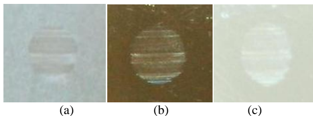
Fig. 3. Scar Images for SAE 20W40 + 10% Vol. CSO + 0.5 % Wt. graphite (a) Ball One; (b) Ball Two; (c) Ball Three
