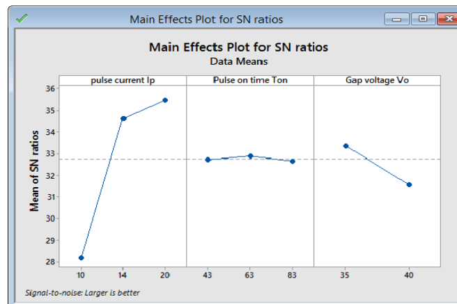
Graph 8: S/N plot for MRR Square tool
