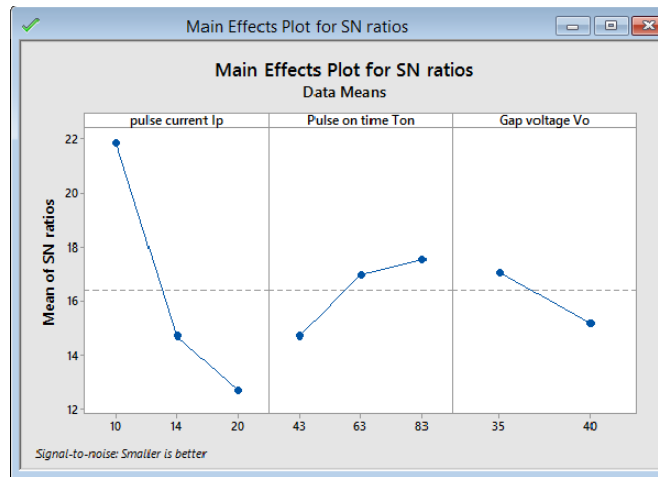
Graph 7.13: S/N ratio plot for TWR Square tool
