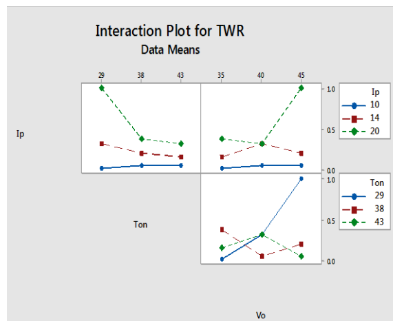
Graph 8: Interaction plot for TWR
