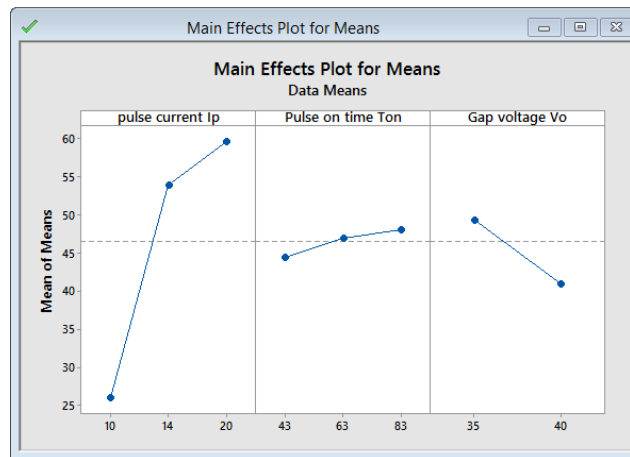
Graph 6: Means plot for MRR for Square tool
