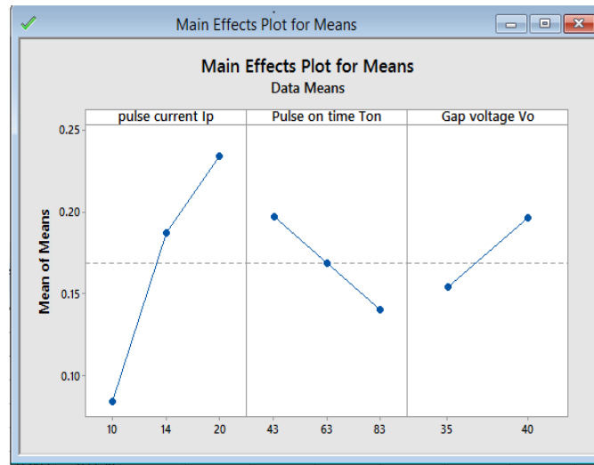
Graph 7.11: Mean plot for TWR Square tool
