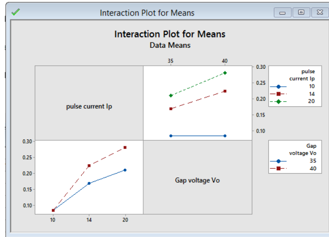
Graph 9: Interaction plot for TWR Square tool
