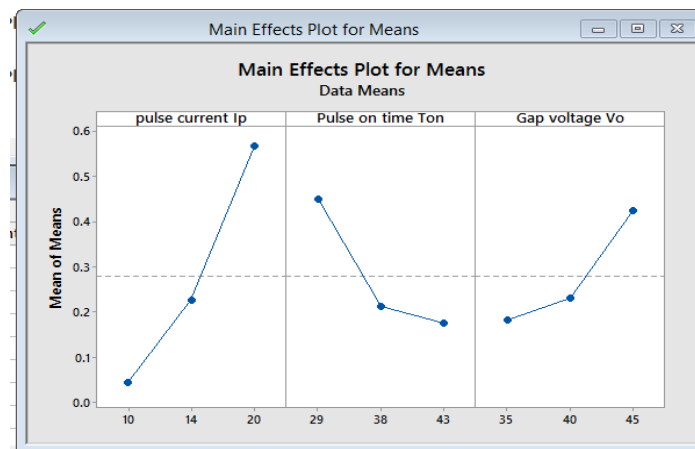
Graph 10: Mean plot for TWR
