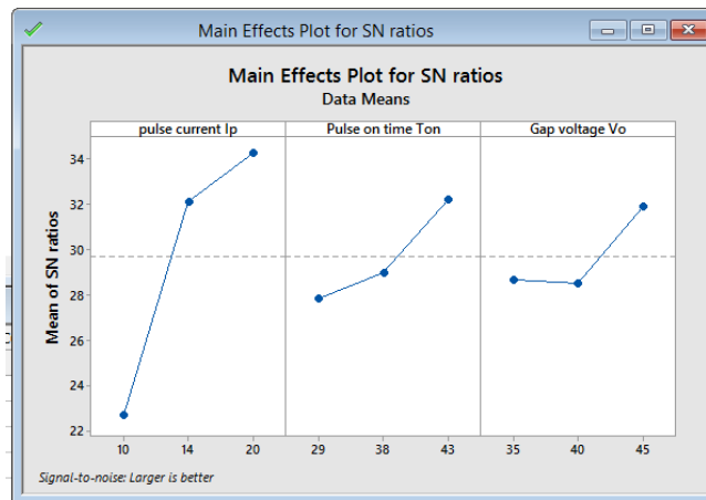
Graph 7: S/N plot for MRR
