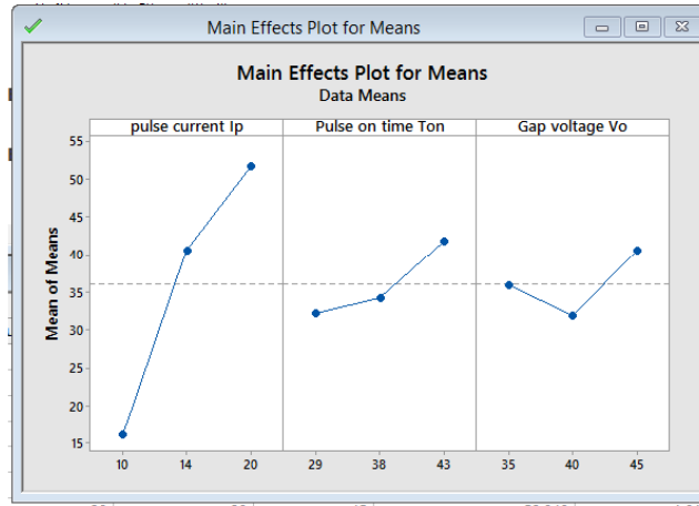
Graph 5: Means plot for MRR
