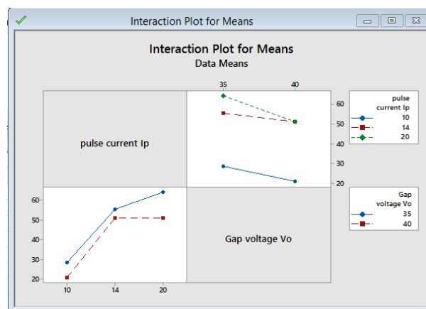
Graph 4: Interaction plots for MRR Square
