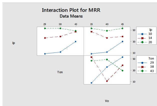
Graph 3: Interaction plots for MRR
