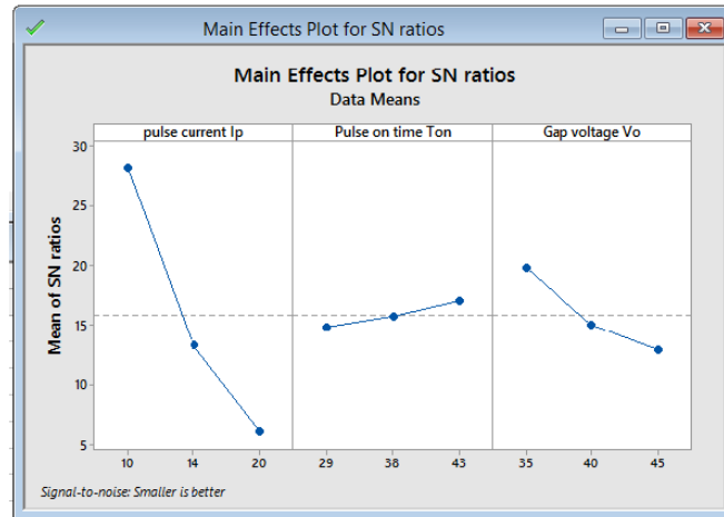
Graph 7.12: S/N ratio plot for TWR
