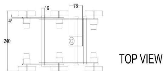
Fig. 4. 2D Drawing of Rocker Bogie Mechanism
