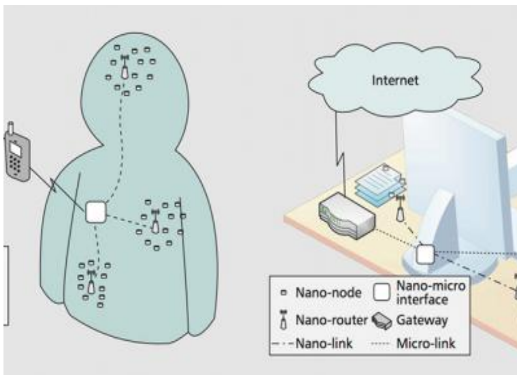
Fig 1. Classical Architecture of Internet of Nano Things (IoNT).
