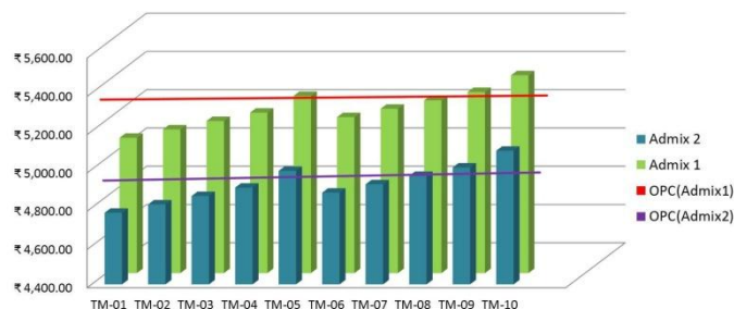
Fig.8. Cost comparison analysis
