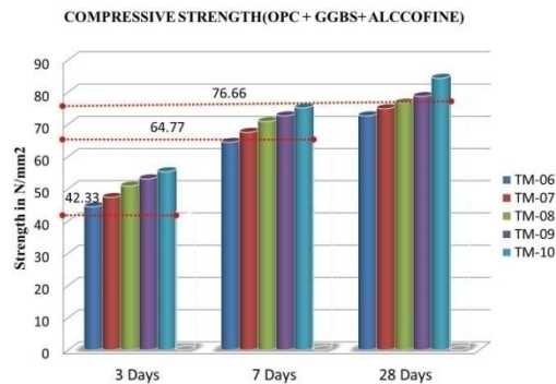
Fig.7. Compressive Strength Analysis(GGBS mixes)
