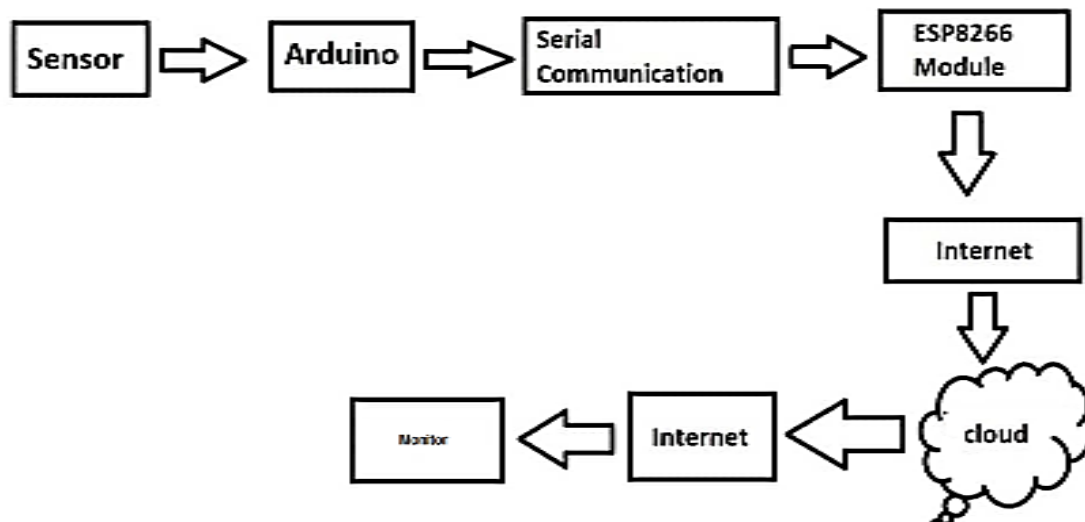
Fig.3: System Flowchart
