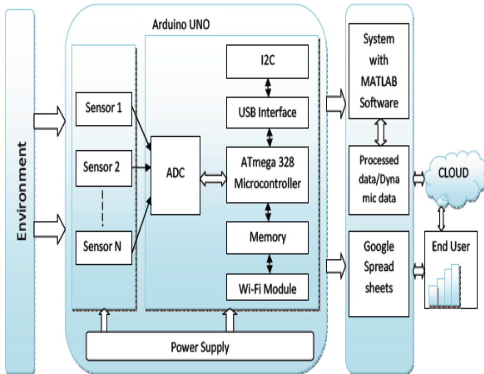
Fig. 4: Schematic diagram of implementation model
