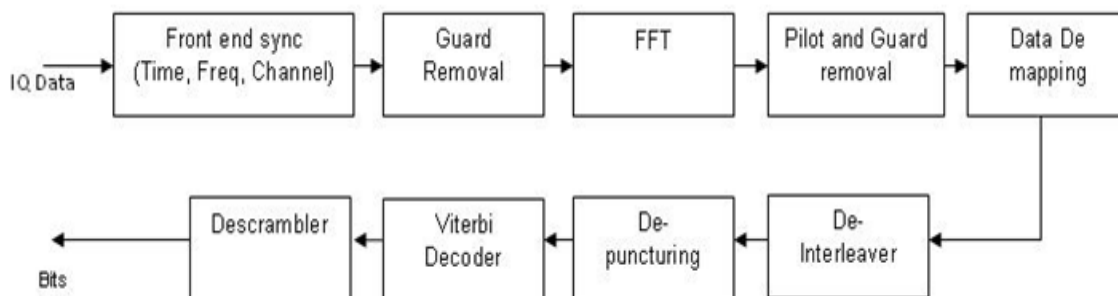
Figure 2. Block Diagram of Receiver of Wireless LAN.
