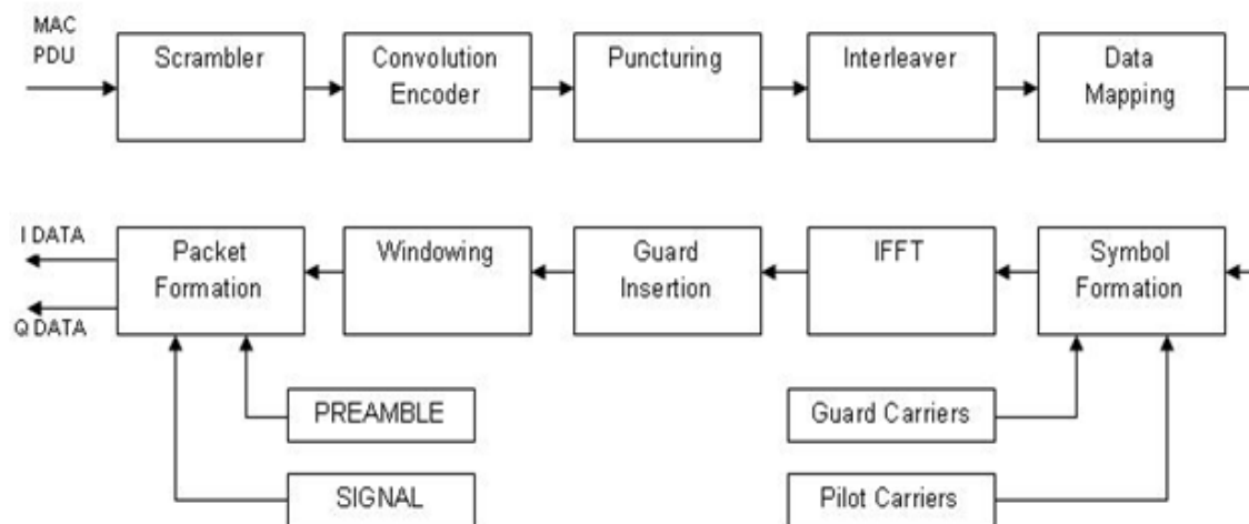
Figure 1. Block Diagram of Transmitter of Wireless LAN.
