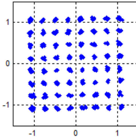
Figure 5. Constellation Diagram of Equalized Signal of Wireless LAN.
