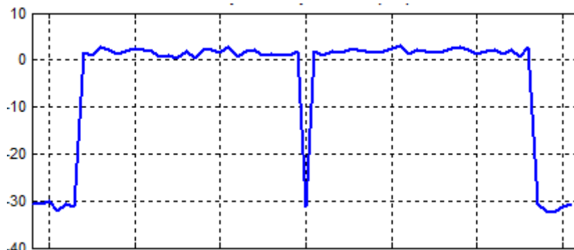
Figure 6. Power Spectrum of Received Signal of Wireless LAN.
