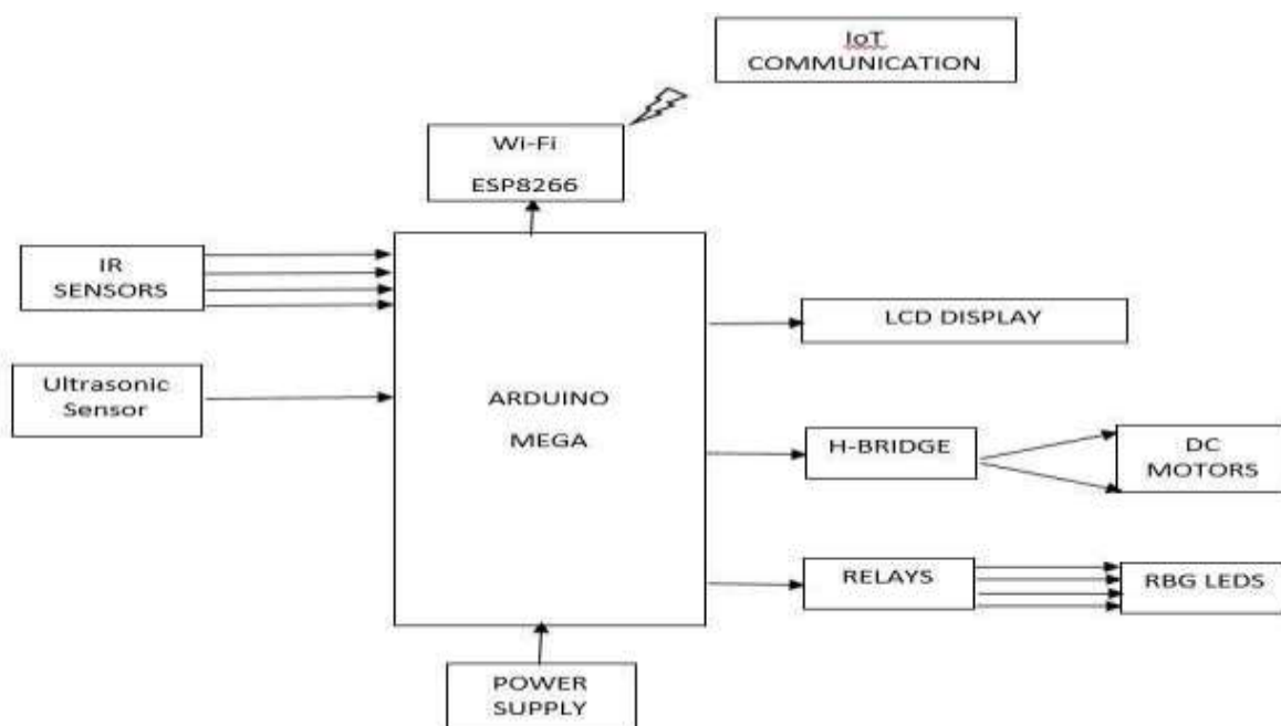
Fig 1. Block diagram
