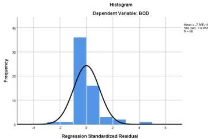
Graph 8: Histogram for BOD through SPSS
