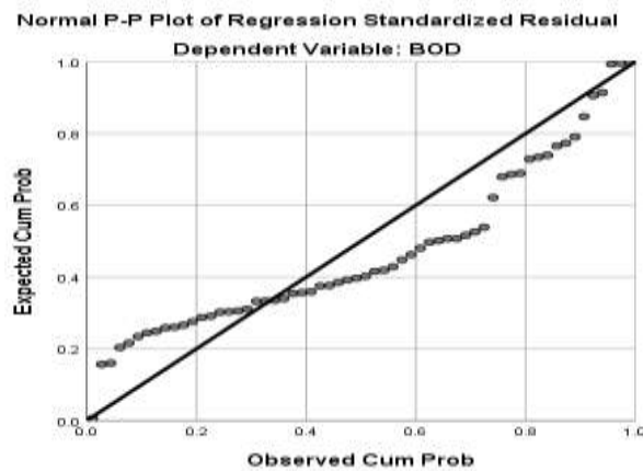
Graph 9: Normal P-P Plot of Regression Standardized Residual through SPSS
