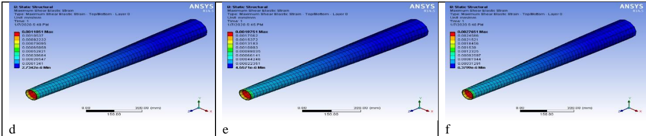
Fig 8: a, b, c: Maximum shear elastic strain for Steel Shaft and d, e, f: for composites at moment 1500 N-m, 2500 N-m and 3500N-m respectively
