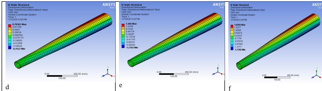
Fig 5: a, b, c: Directional deformation along Y-axis for steel shaft and d,e,f: for composites at moment 1500 N-m, 2500 N-m and 3500 N-m respectively
