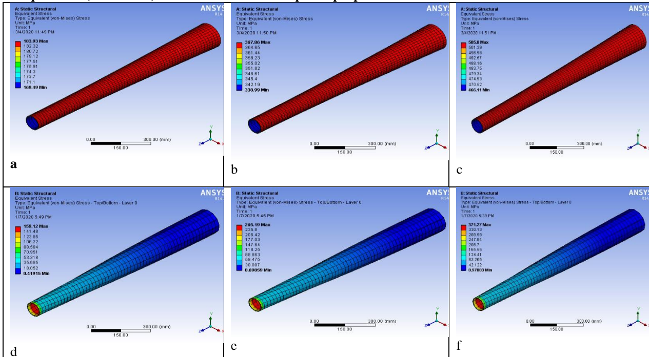
Fig 7: a, b, c: Equivalent stress for steel shaft and d, e, f: for composites at moment 1500 N-m, 2500 N-m and 3500N-m respectively
