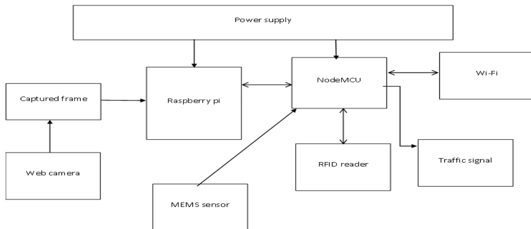
Fig. 1 Block Diagram
