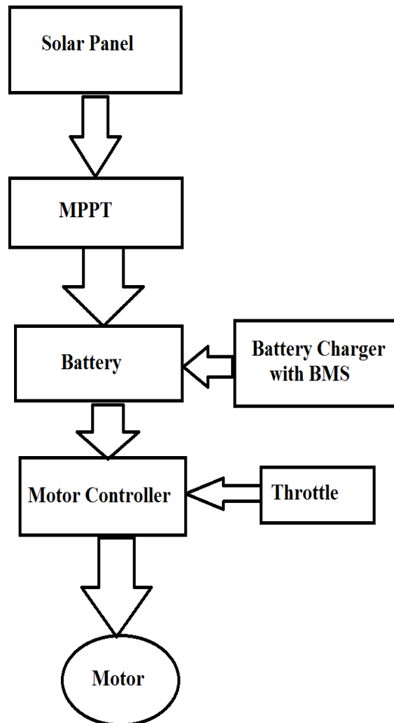
Block diagram of Electrical Circuit
