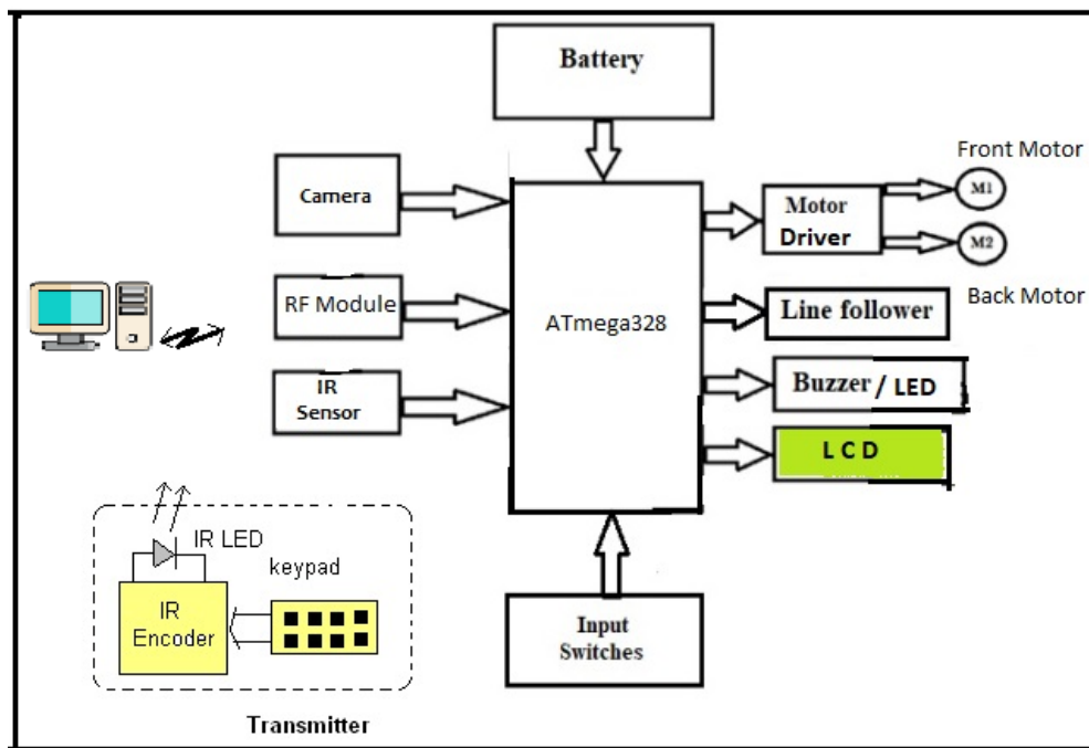
Basic Block Diagram of AGV
