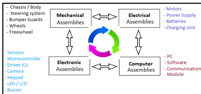
AGVs Sub Assemblies
