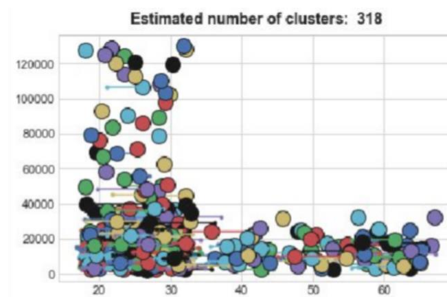
FIGURE 5. Affinity Propagation algorithm generates clusters for the Avg. Money saved each year for touring (Rs.) based on the age attribute. Estimated number of clusters generated is 318.
