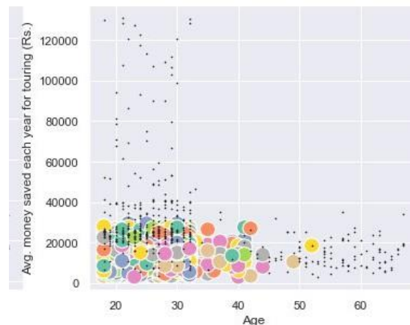
FIGURE 4. DBSCAN algorithm generates clusters for the Avg. Money saved each year for touring (Rs.) based on the age attribute.
