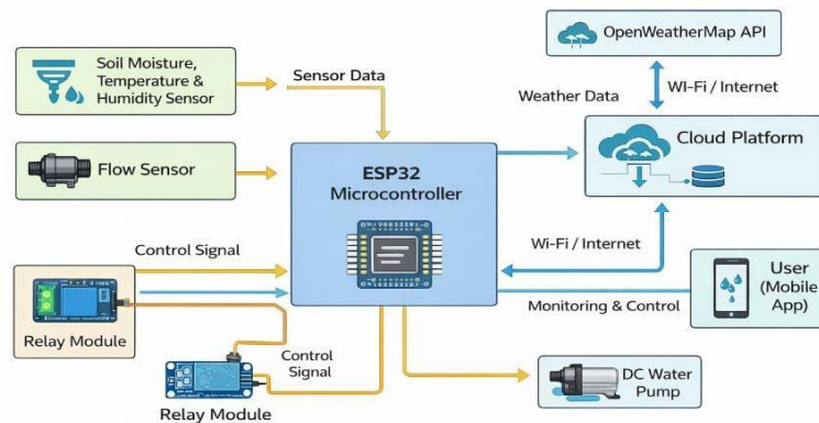
Fig 3.1 Block Diagram
