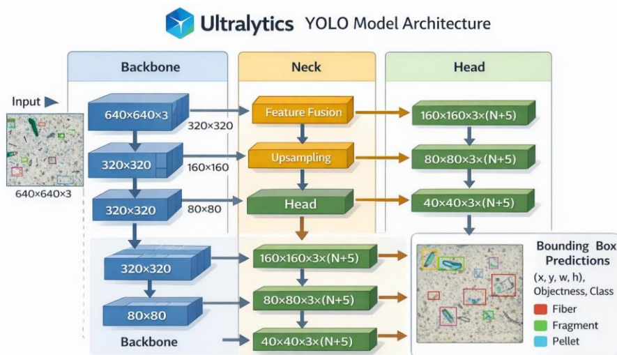
Fig 2: YOLO Architecture
