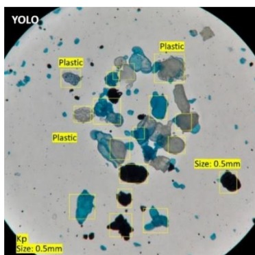
Fig 1: Plastic detection
